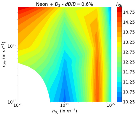
Fig. 4: Runaway electron generation during STEP mitigated disruptions - Scan in Neon and D_2 injected quantities
