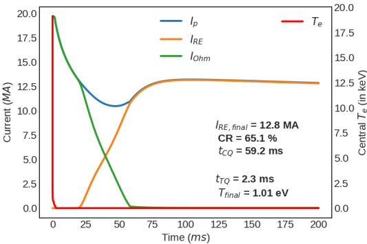
Fig. 3: Runaway electron generation during a STEP mitigated disruption with Neon and D_2 impurity injections ( n_{Ne} = 5 \times 10^{19} \text{ m}^{-3} , n_{D2} = 10^{21} \text{ m}^{-3} , f_{\text{rad}} = 93\% )
