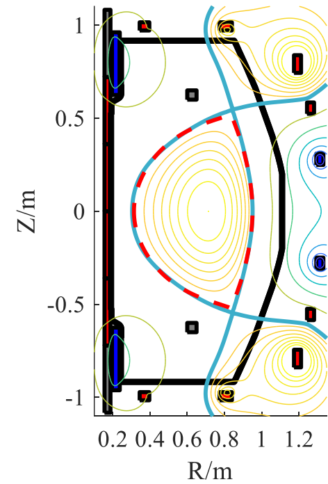
negative triangularity
